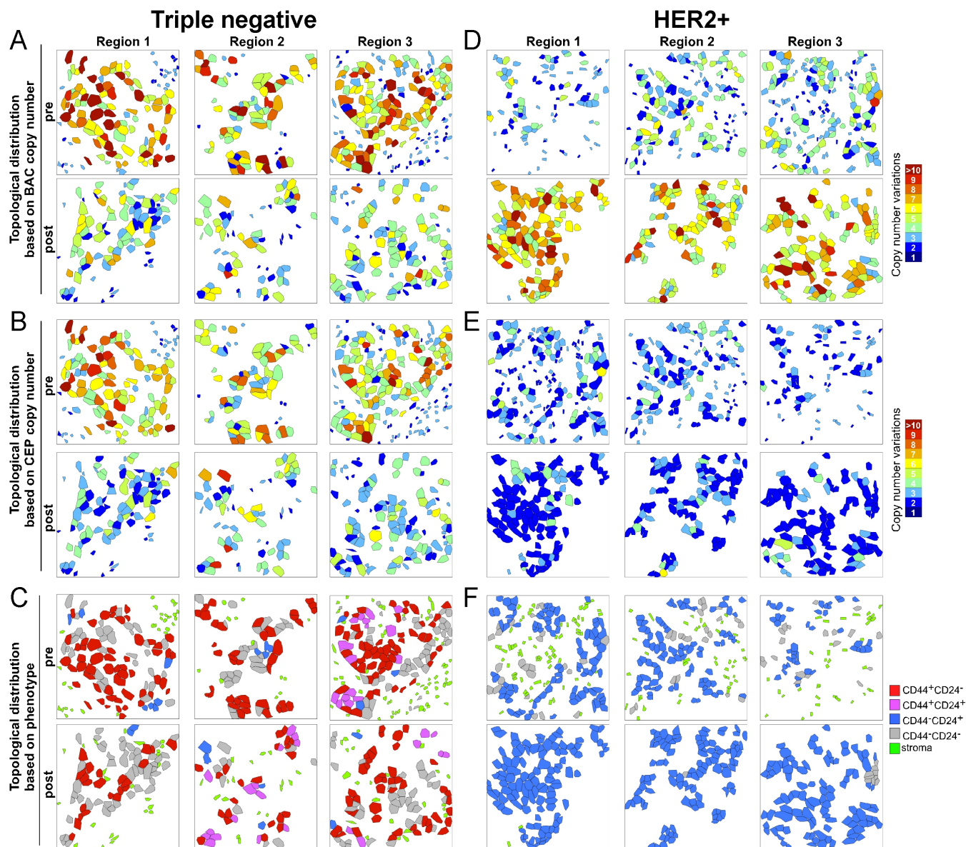
Figure S4. Analysis of the topologic distribution of genetically and phenotypically divergent cells within tumors. Related to Figure 3.
