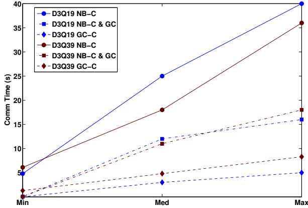
Figure 9. Time in seconds spent in communication for the min, median and max nodes at various optimization levels. For the case of 133,000 nodes, each individual nodes ran out of memory due to the addition of the fourth ghost cell, and thus could not complete the simulation.
