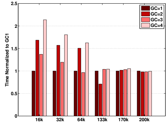
(b) D3Q39
