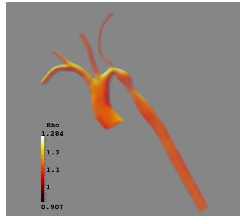
Figure 1. Fluid density in the aorta.
